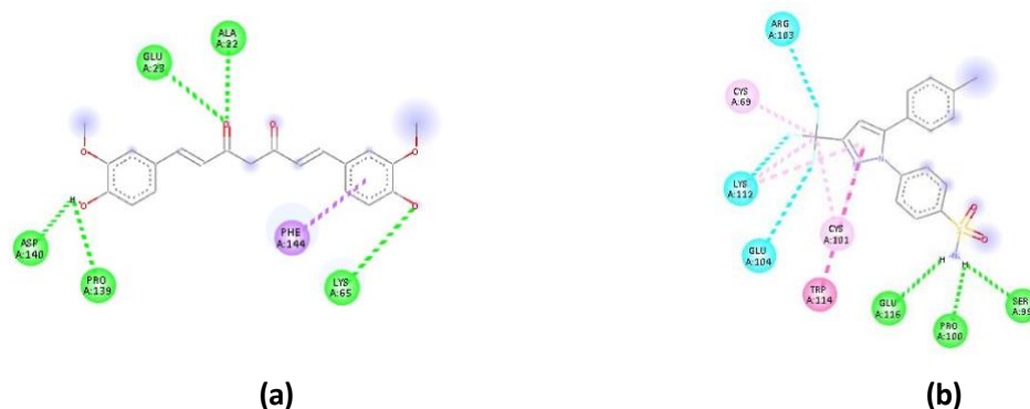
Fig. 2. Two-dimensional molecular interaction maps of (a) curcumin and (b) celecoxib with the TNF- \alpha receptor.
